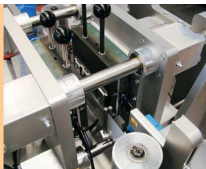
Contour sealing of the bags
